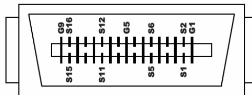
Front-View CX4 Connector
